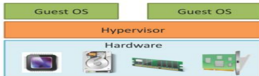
Type-1 Hypervisor
