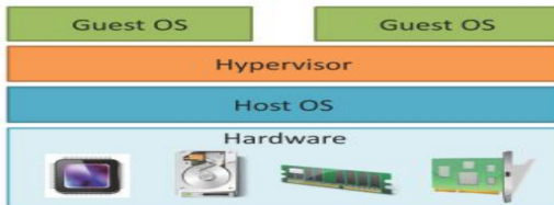
Type-2 Hypervisor
